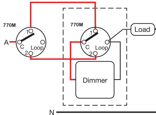
Two-way wiring diagram
